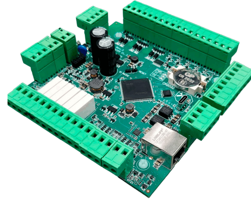
Embedded HVAC controller
